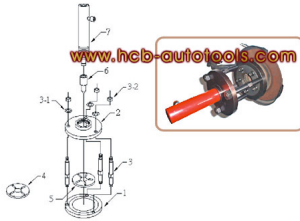
THE ILLUSTRATION OF TOOL
